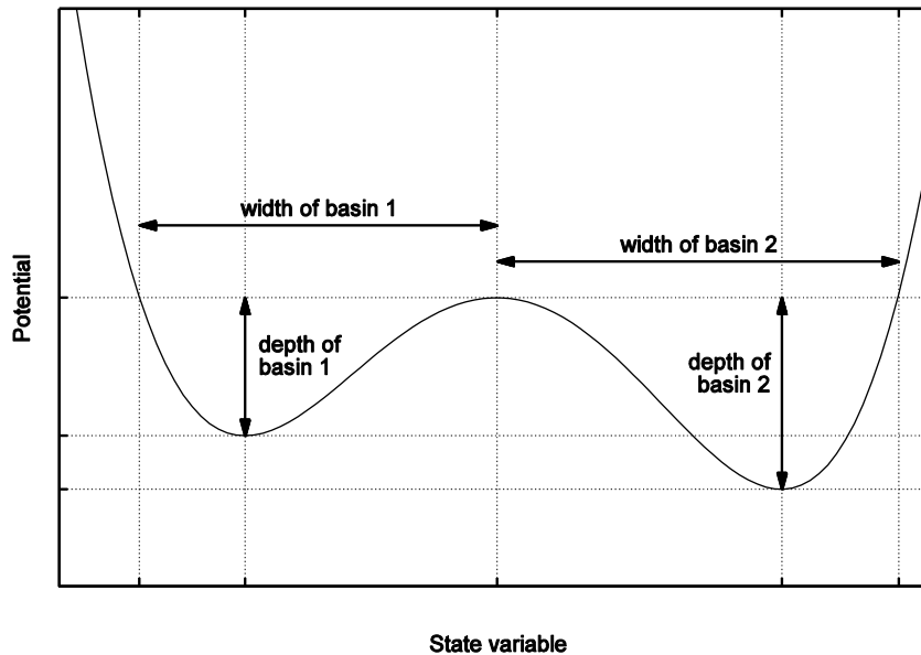
Fig. 5. Measures of resilience for one dimensional potential.
